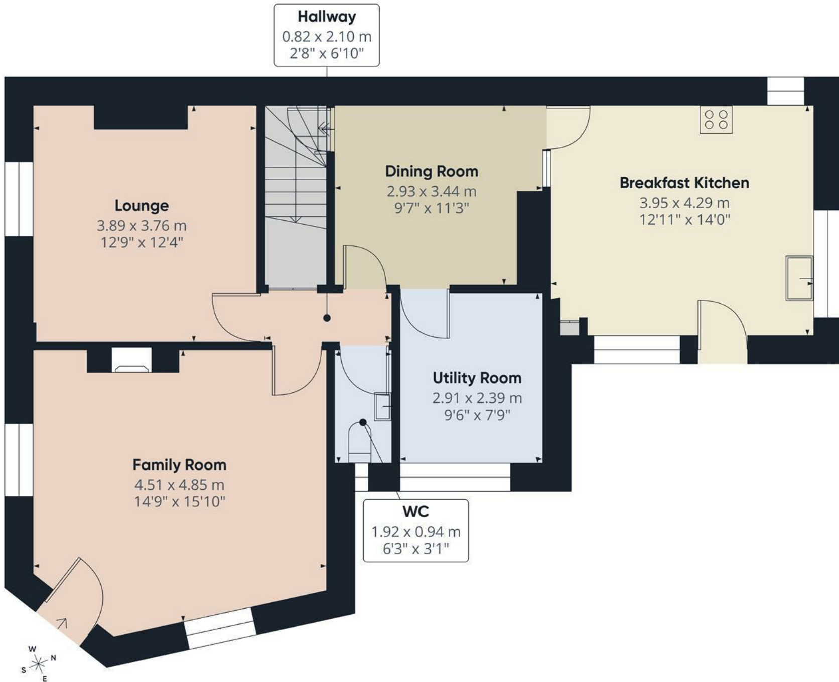
Floor 0
