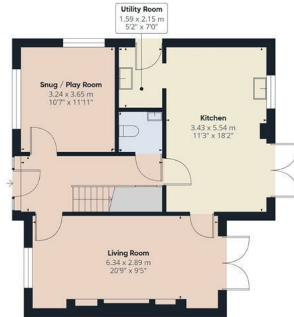
Floor 0 Building 1
