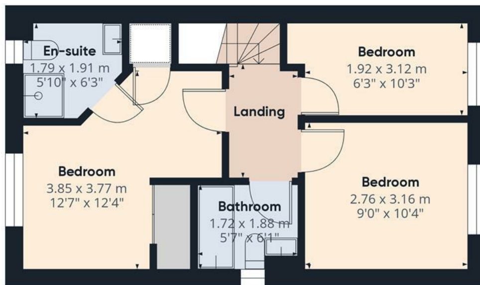
Floor 1
