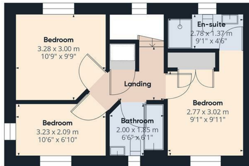
Floor 1 Building 1
